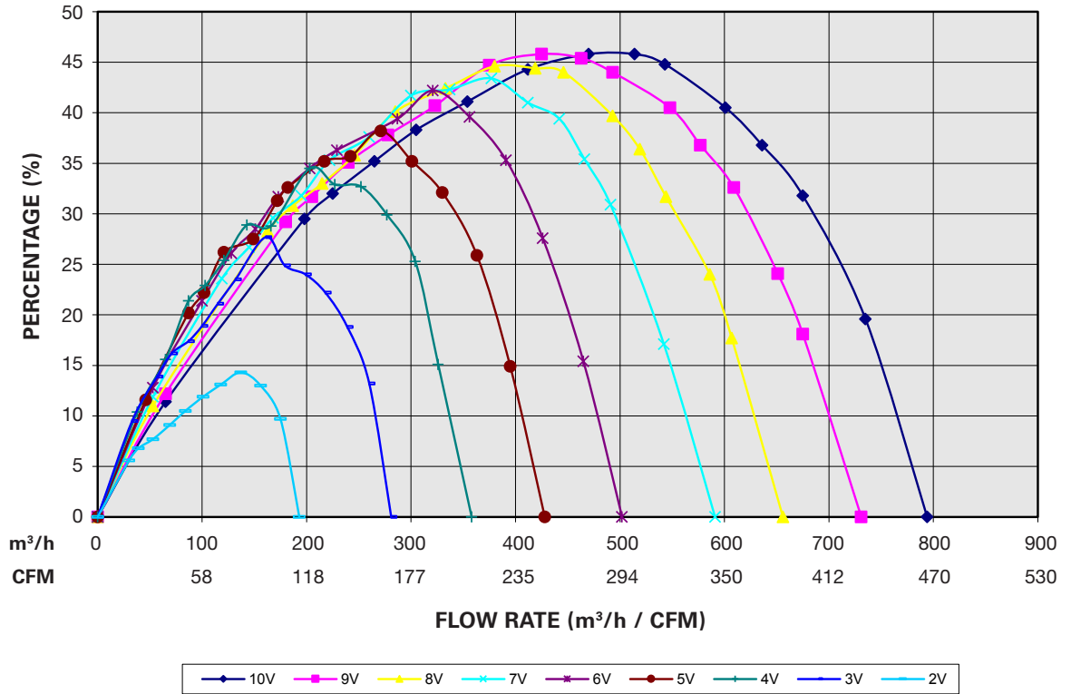
STATIC EFFICIENCY CHART
