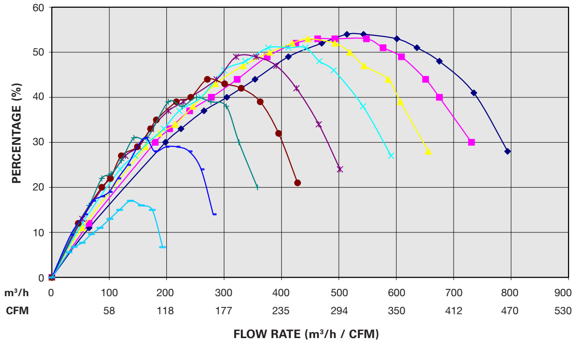
TOTAL EFFICIENCY CHART
