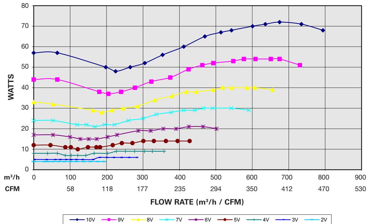
POWER CONSUMPTION
